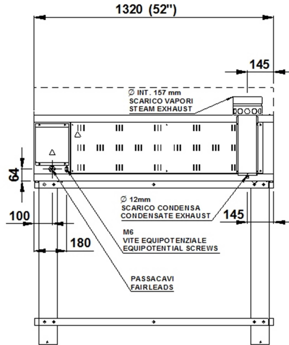
REAR VIEW
