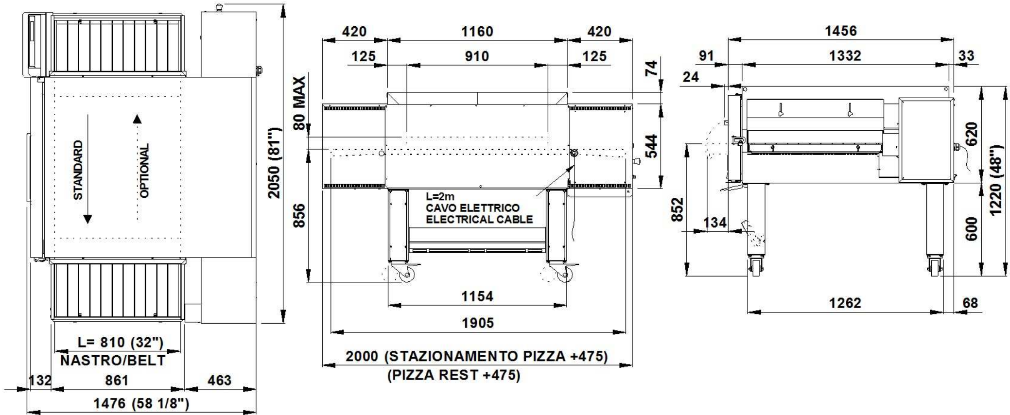
TOP VIEW
